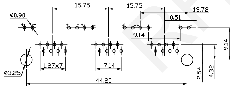
PCB Layout
